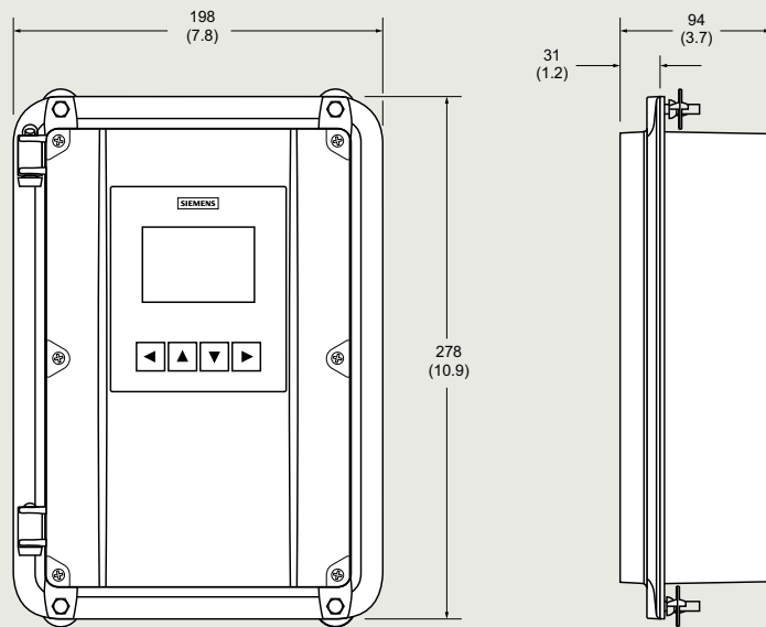
SITRANS LT500, dimensions in mm (inch)
